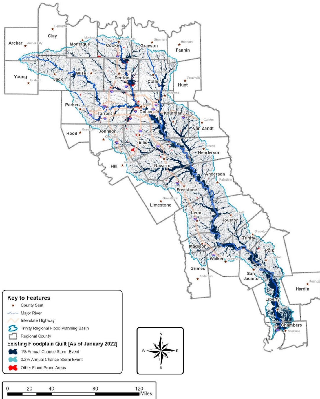
Figure 2.5: Existing Condition Floodplain Quilt
